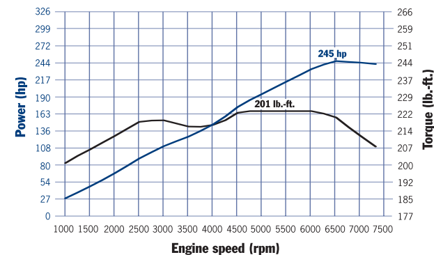
Boxster: 201 lb.-ft. at 4600–6000 rpm, 245 hp at 6500 rpm
