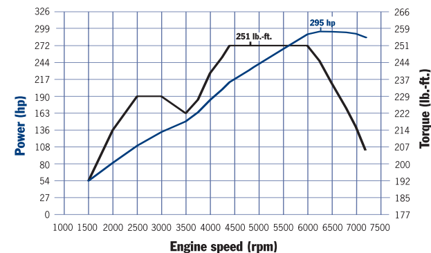
Boxster S: 251 lb.-ft. at 4400–6000 rpm, 295 hp at 6250 rpm
