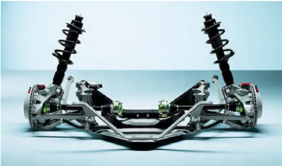
MacPherson rear axle with suspension struts and transverse links (Boxster S)
